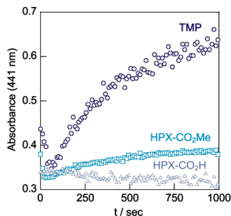
Figure 6. Formation of ferric N -oxide products (with \lambda_{\max} = 441 nm) for P = TMP (○), HPX—CO 2 Me (□), and HPX—CO 2 H (△) at [Fe III ] = 9.0 × 10 -6 M and [m-CPBA] = 2.7 × 10 -5 M at -20 °C in toluene.
