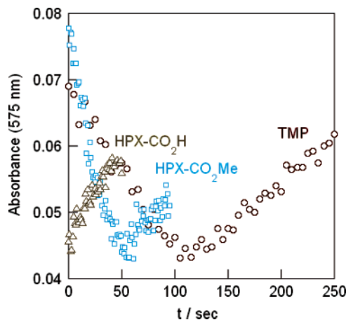
Figure 2. Selected time-resolved data for the disappearance of (P)Fe III (OH) ( 9.0 \times 10^{-6} M; \lambda_{\text{max}} = 575 nm) in reactions with 3.5 \times 10^{-4} M m -CPBA at -40 °C in CH 2 Cl 2 to make (P)Fe III (O 2 COAr) and subsequent O–O bond heterolysis [P = TMP (○), HPX-CO 2 Me (□), HPX-CO 2 H (△)].
